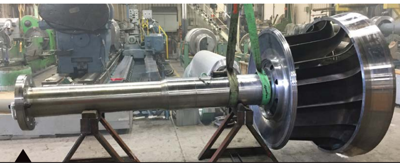
MACHINED FRANCIS RUNNER Installed on new turbine shaft
