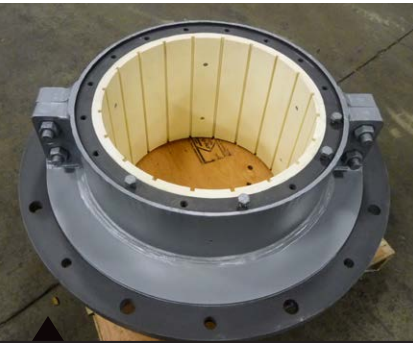
THORDON SXL Turbine guide bearing
